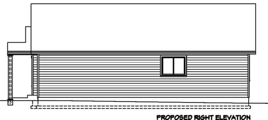
PROPOSED RIGHT ELEVATION
