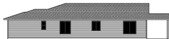
RIGHT SIDE ELEVATION
