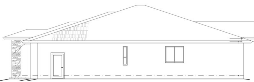
LEFT ELEVATION
