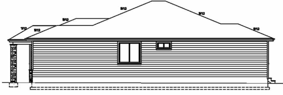
RIGHT ELEVATION SCALE 1/8"=1'-0"
