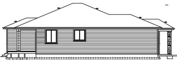
LEFT ELEVATION SCALE 1/8"=1'-0"
