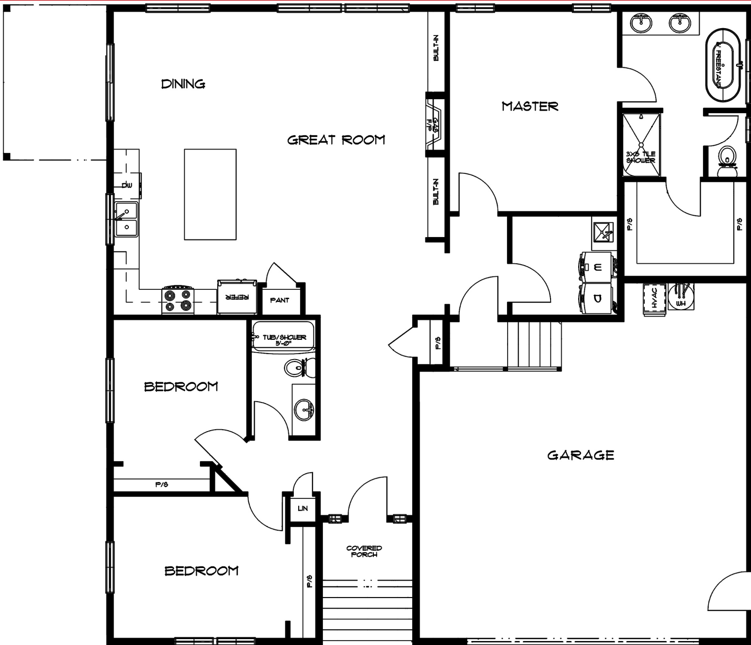
FLOOR PLAN AREA 1138 SF
