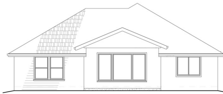
REAR ELEVATION
