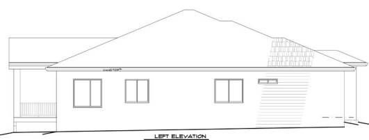
LEFT ELEVATION
