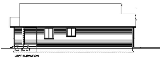
LEFT ELEVATION
