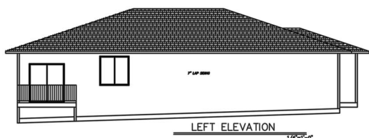
LEFT ELEVATION
