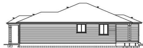
RIGHT ELEVATION SCALE 1/8" = 1'-0"
