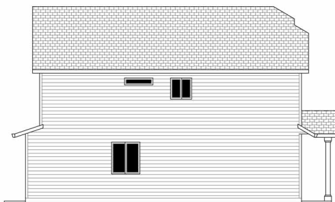
LEFT SIDE ELEVATION
