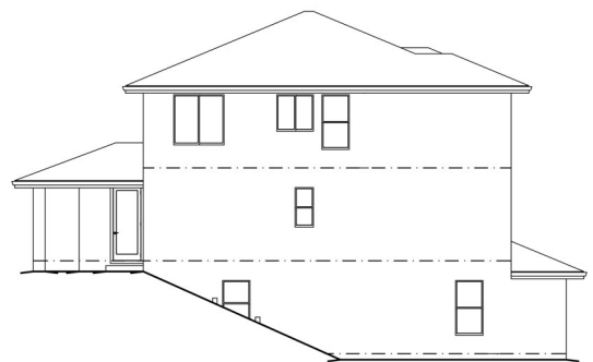
LEFT ELEVATION
