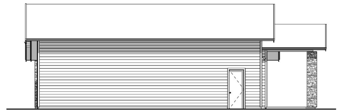
Left Elevation
