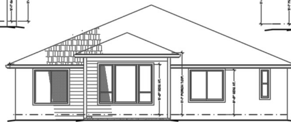
REAR ELEVATION
