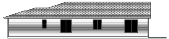
RIGHT SIDE ELEVATION
