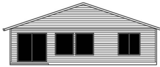
REAR ELEVATION
