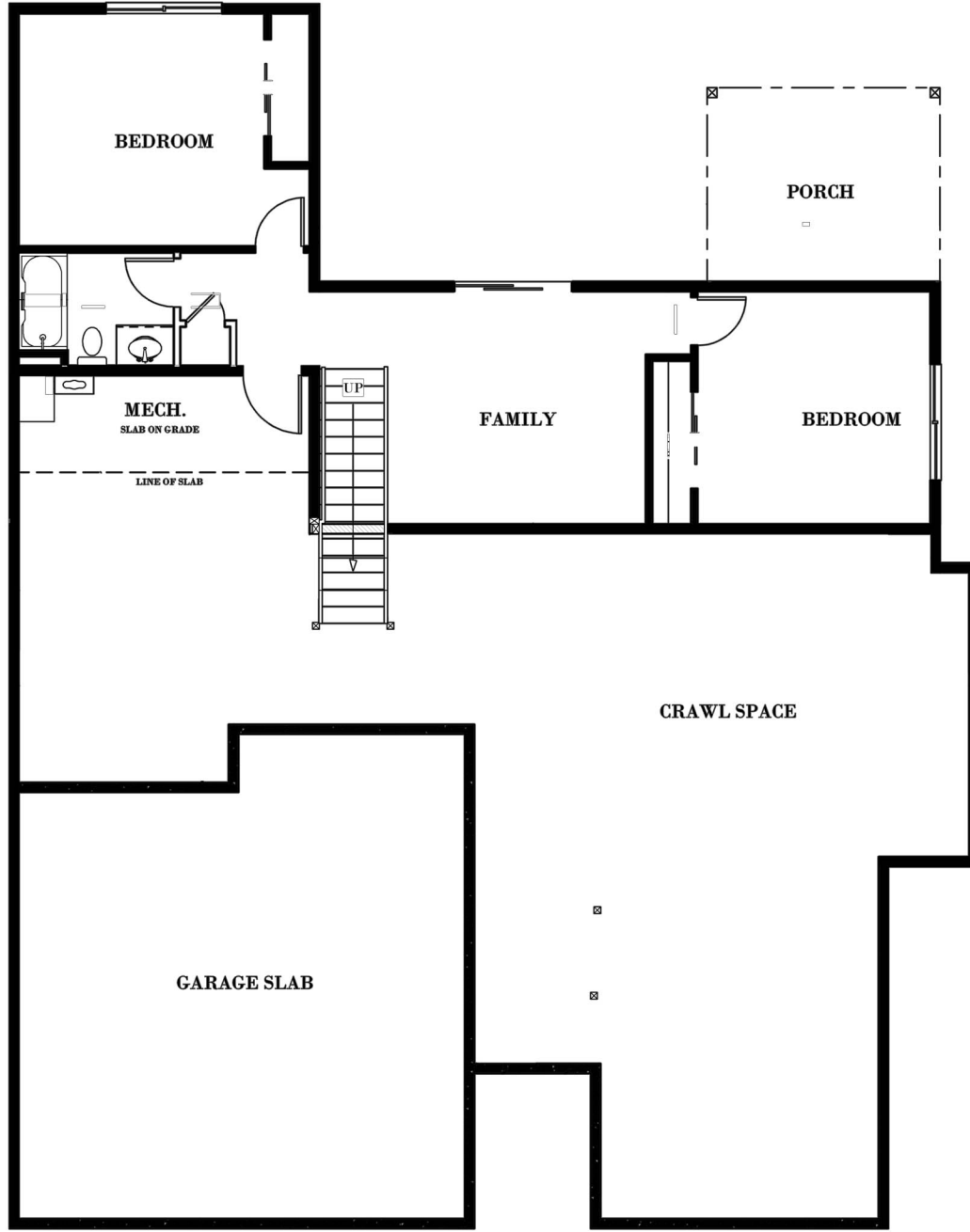
LOWER FLOOR PLAN
